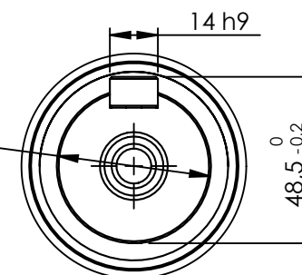
DETAIL X SCALE 1 : 2
