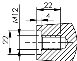
SECTION A-A 4 Holes to baseplate connection SCALE 1 : 2
